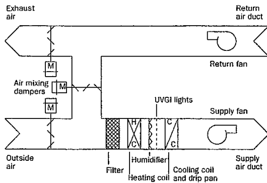
Figure 1: Schematic diagram of a typical HVAC system
